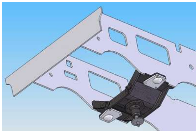
Drawing of bogie bolster (dark grey component) shown fitted to front of frames. Drawn by Kevin West.
